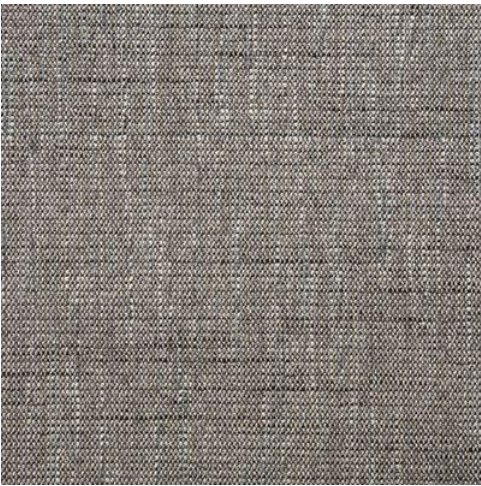
Shale
